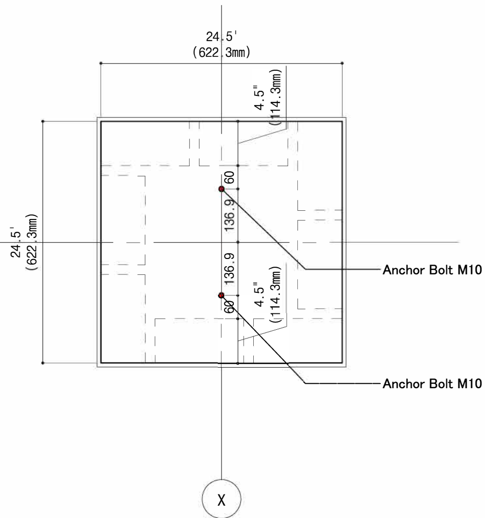
Anchor Bolt Detail Type A+B
